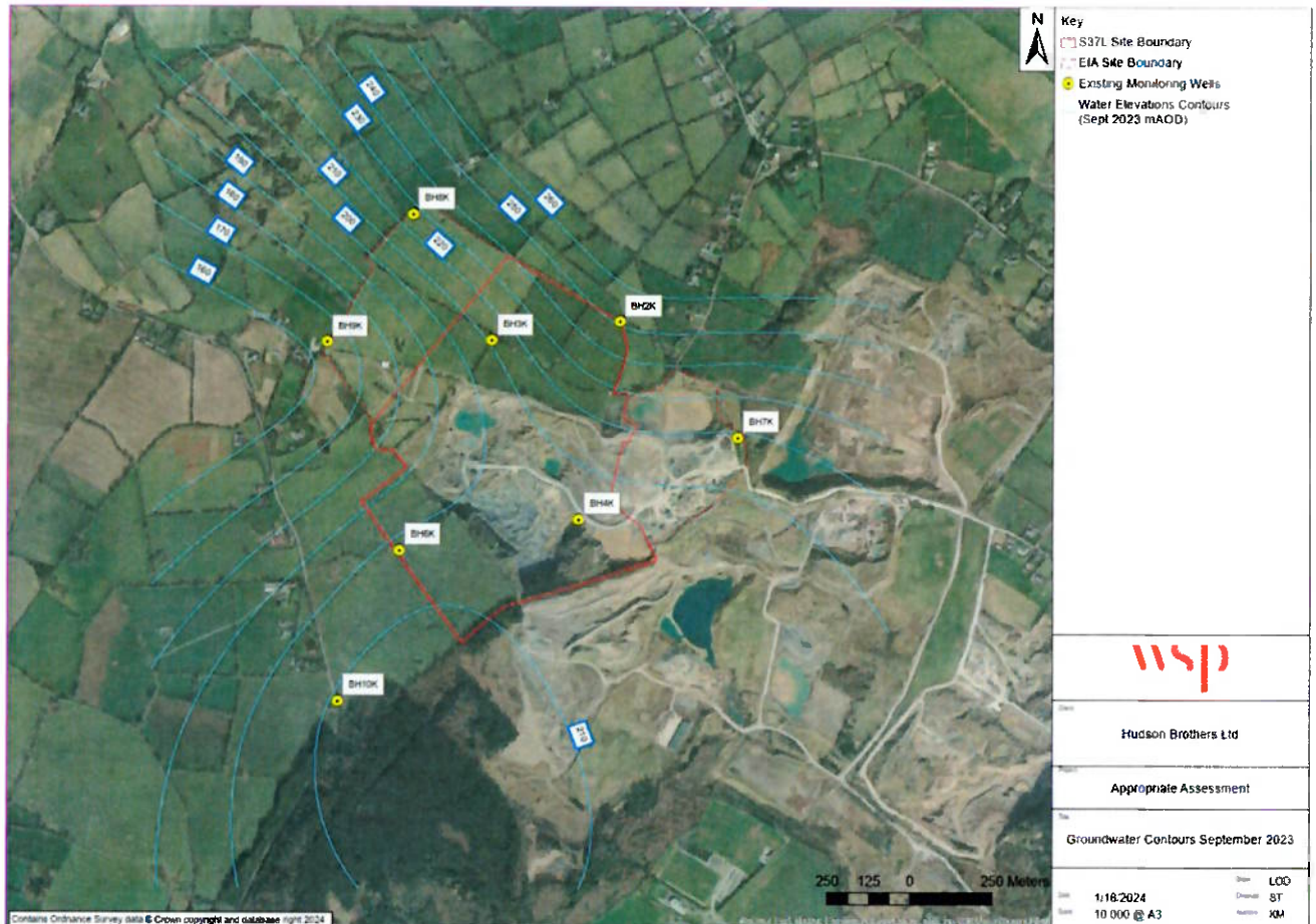
Figure 2-10 – Groundwater Contours September 2023
