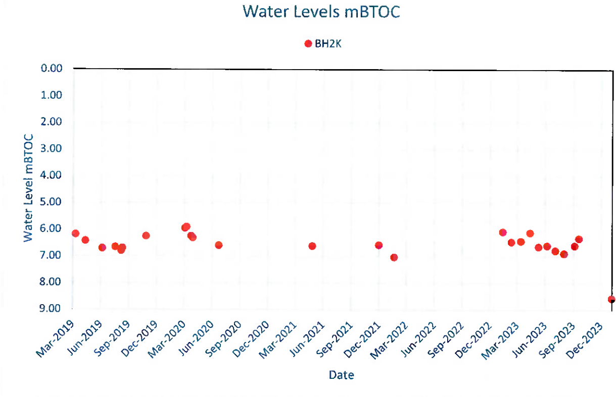
Figure 5-1 – Groundwater Levels at Monitoring Well BH2K
