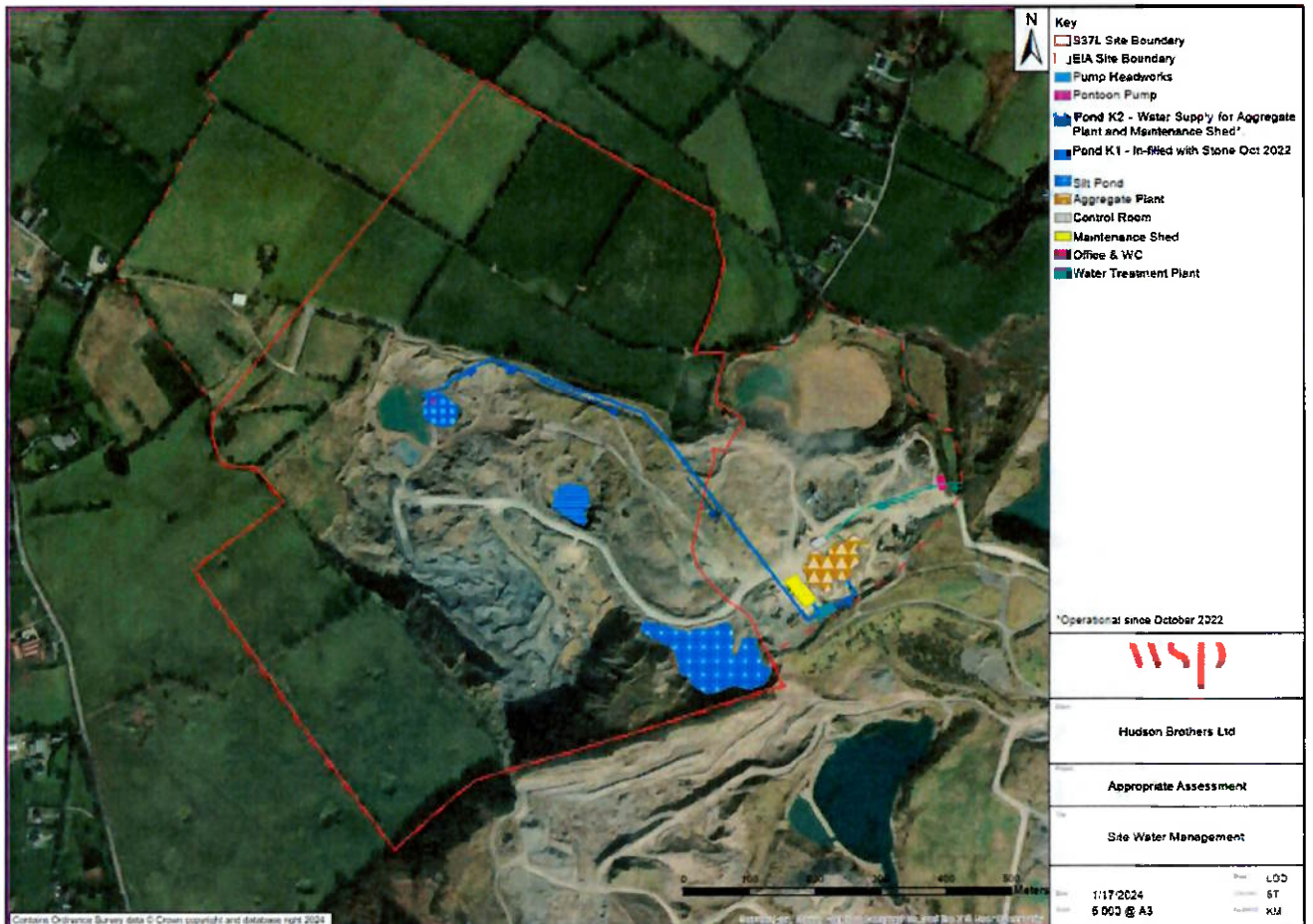
Figure 2-6 - Site Water Management
