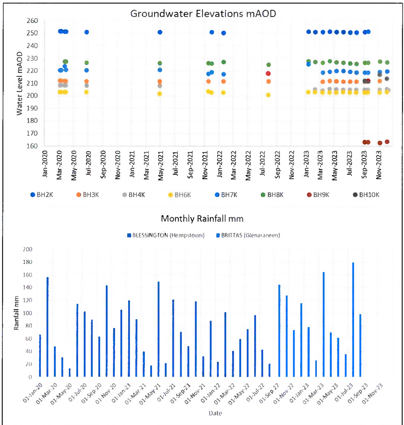
Figure 2-9 - Groundwater Elevations Over Period 2020-2023
