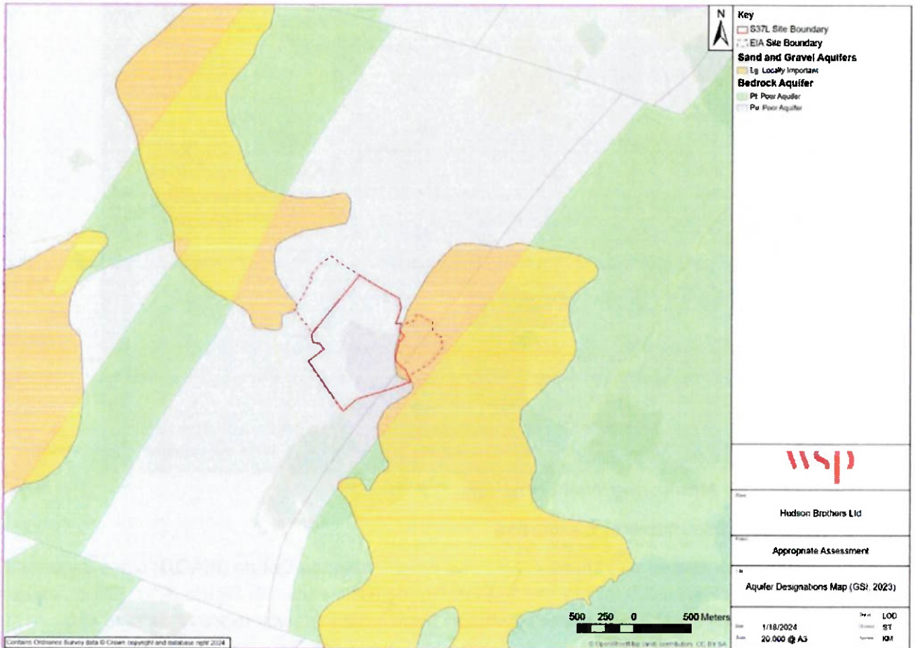
Figure 2-7 - Aquifer Designation Map (GSI, 2023)
